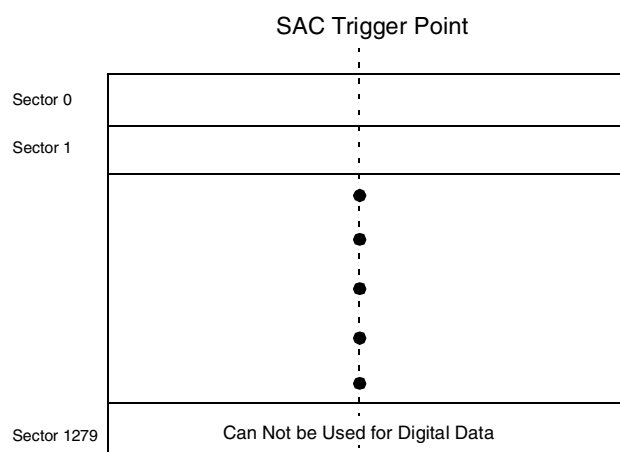
Figure 3 Memory Map.
