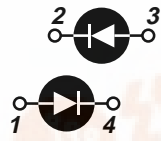
Anti-Parallel APT2X60D30J
