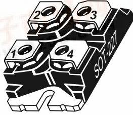
Parallel APT2X61D30J
