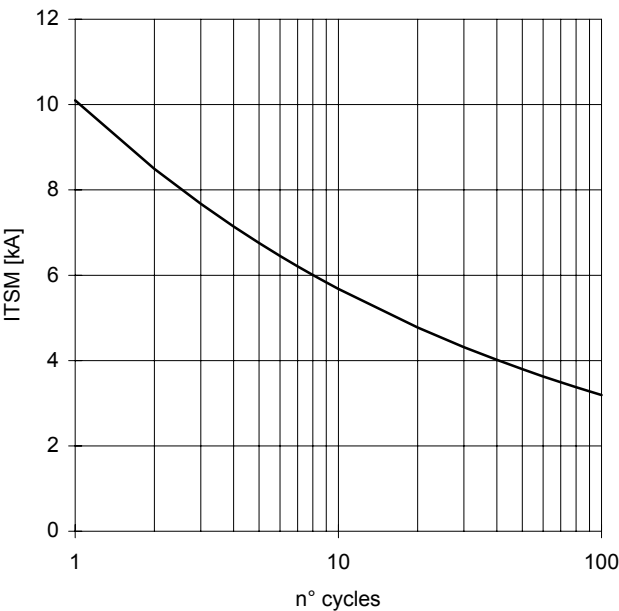
SURGE CHARACTERISTIC T_j = 175^\circ\text{C}
