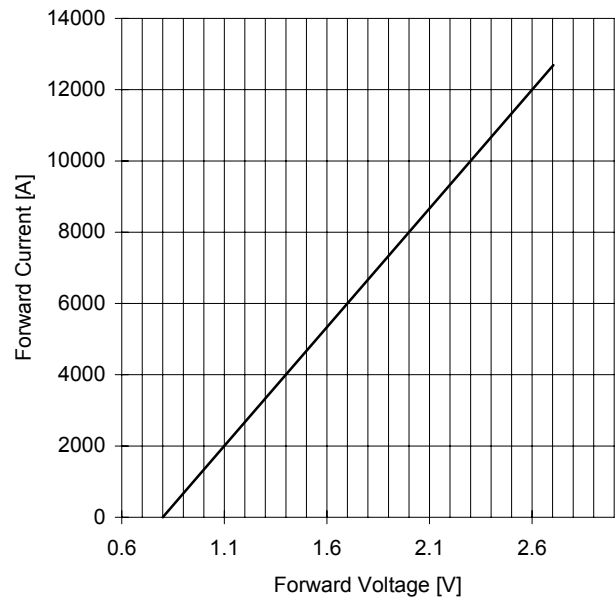
FORWARD CHARACTERISTIC Tj = 150 °C
