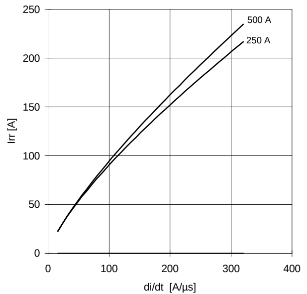
REVERSE RECOVERY CURRENT T_j = 125\text{ }^{\circ}\text{C}
