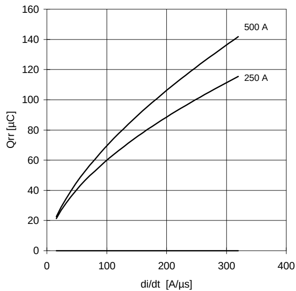
REVERSE RECOVERY CHARGE T_j = 125\text{ }^{\circ}\text{C}
