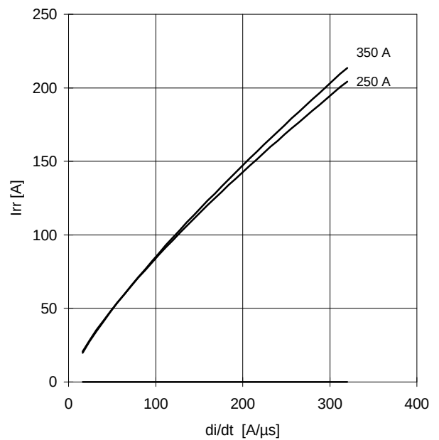
REVERSE RECOVERY CURRENT T_j = 150\text{ }^{\circ}\text{C}
