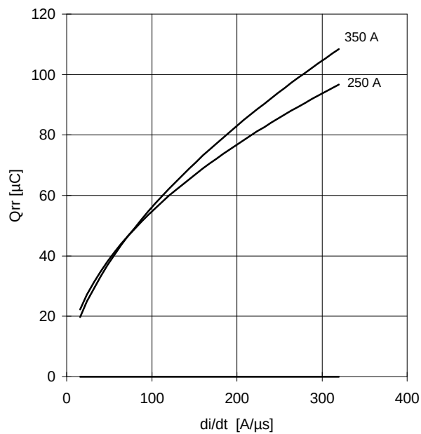
REVERSE RECOVERY CHARGE T_j = 150\text{ }^{\circ}\text{C}
