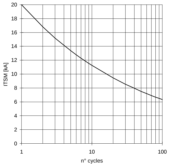
SURGE CHARACTERISTIC T_j = 125^\circ\text{C}
