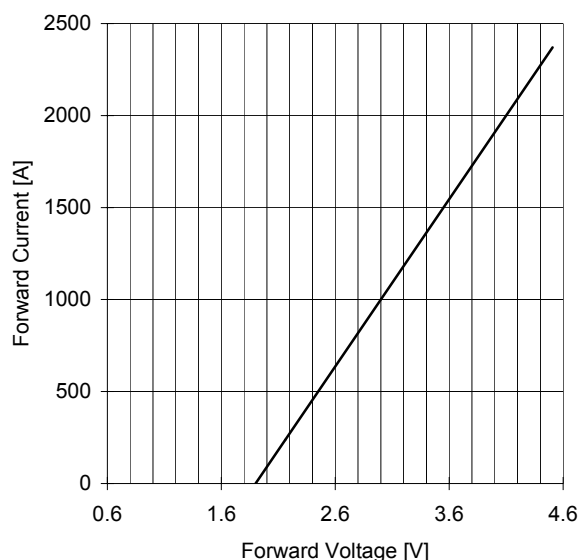
FORWARD CHARACTERISTIC T_j = 125^\circ\text{C}
