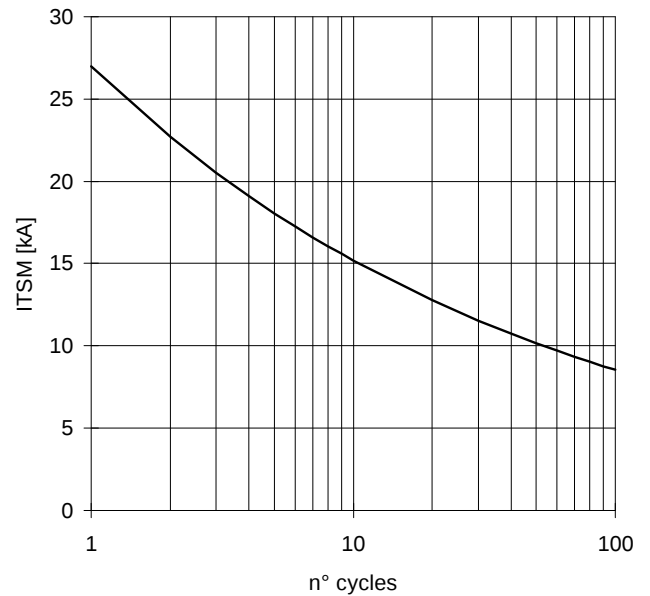
SURGE CHARACTERISTIC T_j = 150^\circ\text{C}
