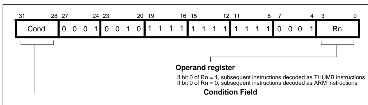
Figure 4-2: Branch and Exchange instructions
