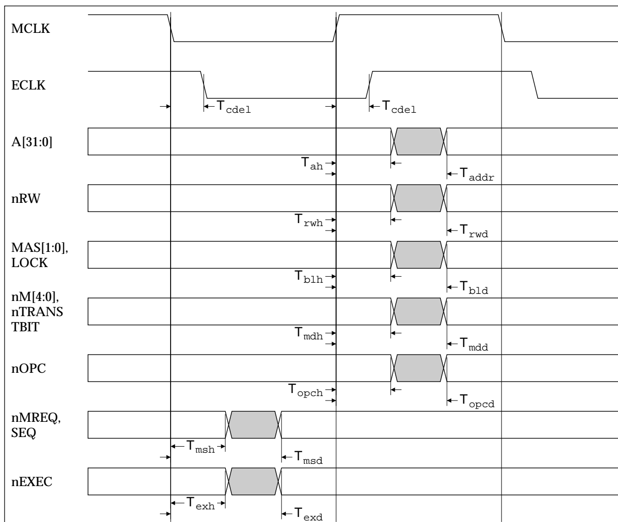
Figure 12-1: General timings
