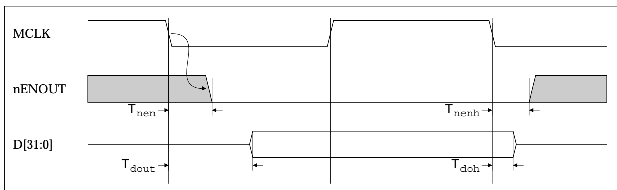
Figure 12-5: Bidirectional data write cycle
