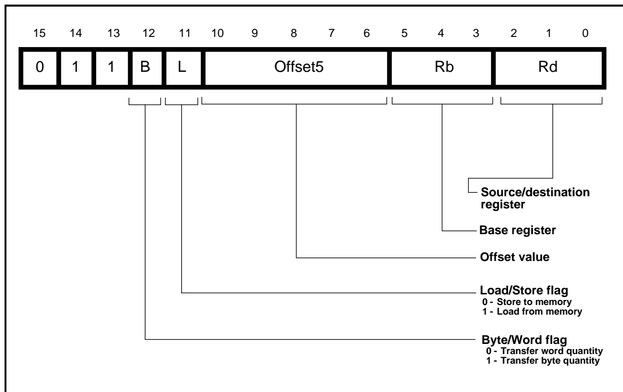
Figure 5-10: Format 9
