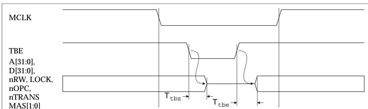
Figure 12-8: Output 3-state time
