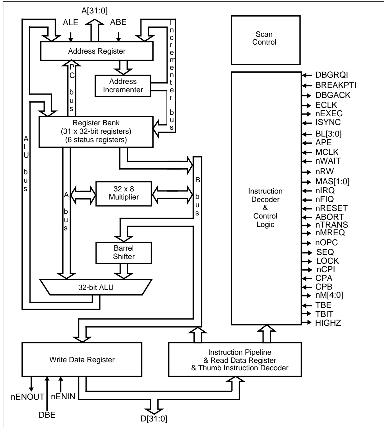
Figure 1-2: ARM7TDMI core
