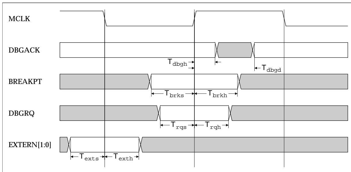
Figure 12-14: Debug timing
