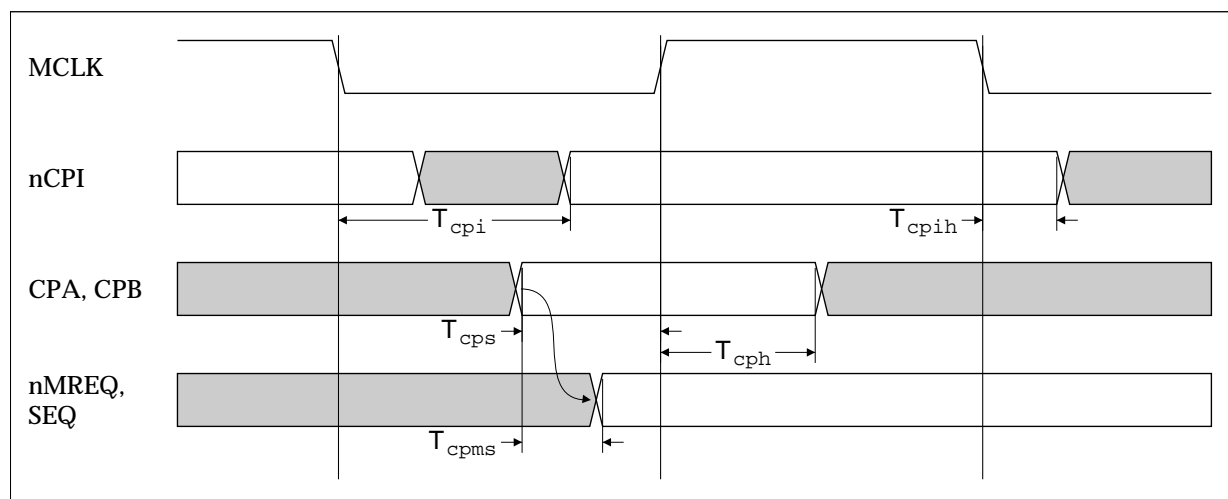
Figure 12-12: Coprocessor timing
