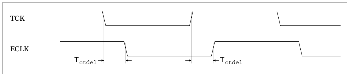
Figure 12-16: TCK-ECLK relationship
