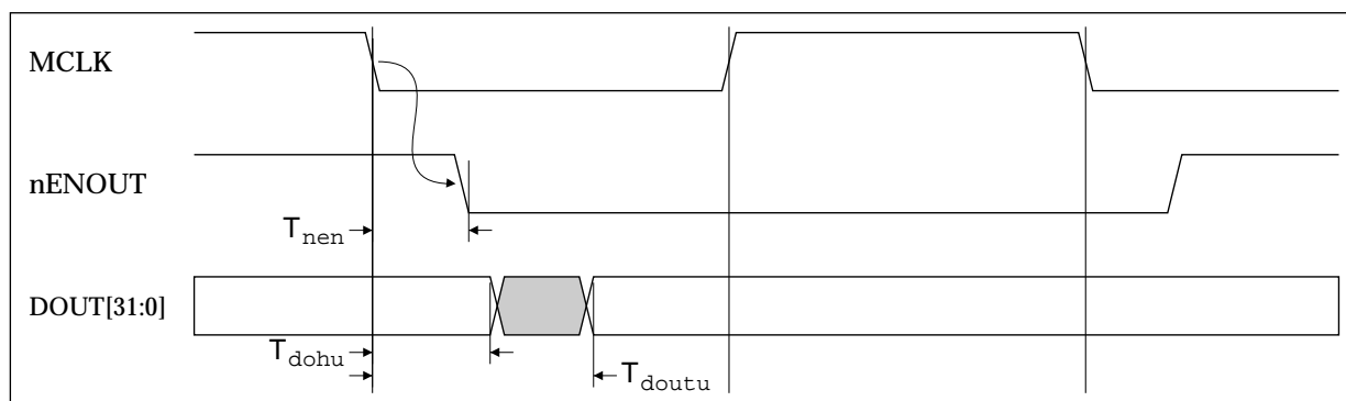
Figure 12-9: Unidirectional data write cycle
