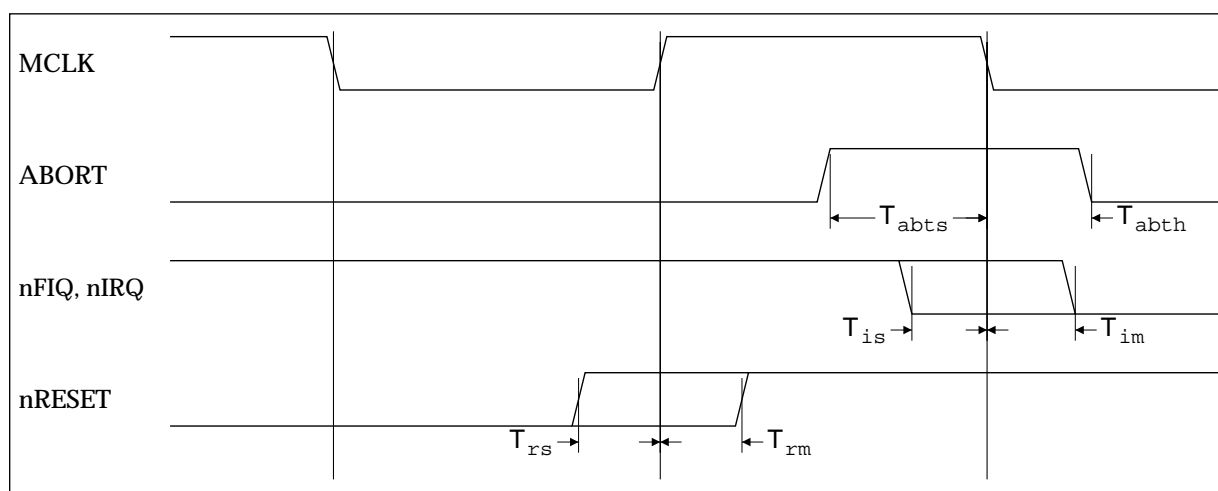
Figure 12-13: Exception timing
