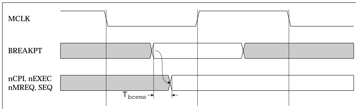
Figure 12-15: Breakpoint timing
