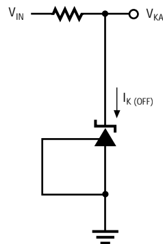
Figure 1c. Test Circuit 3
