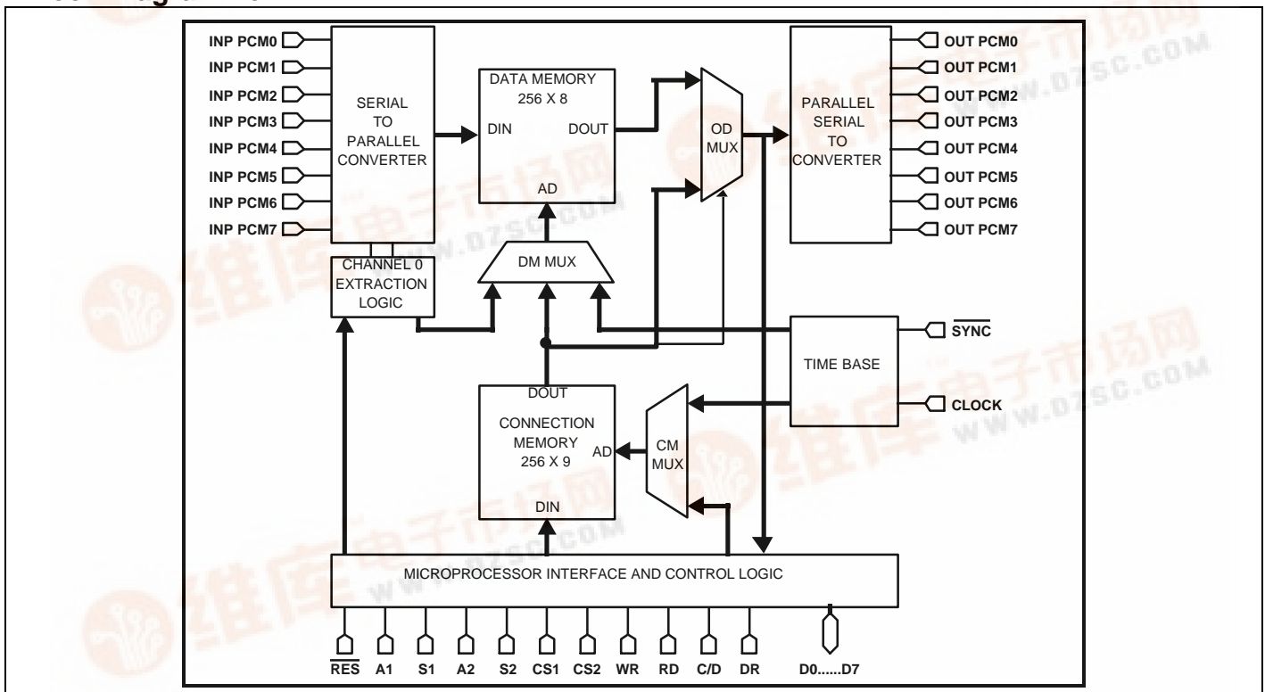
Figure 1: Block Diagramme
