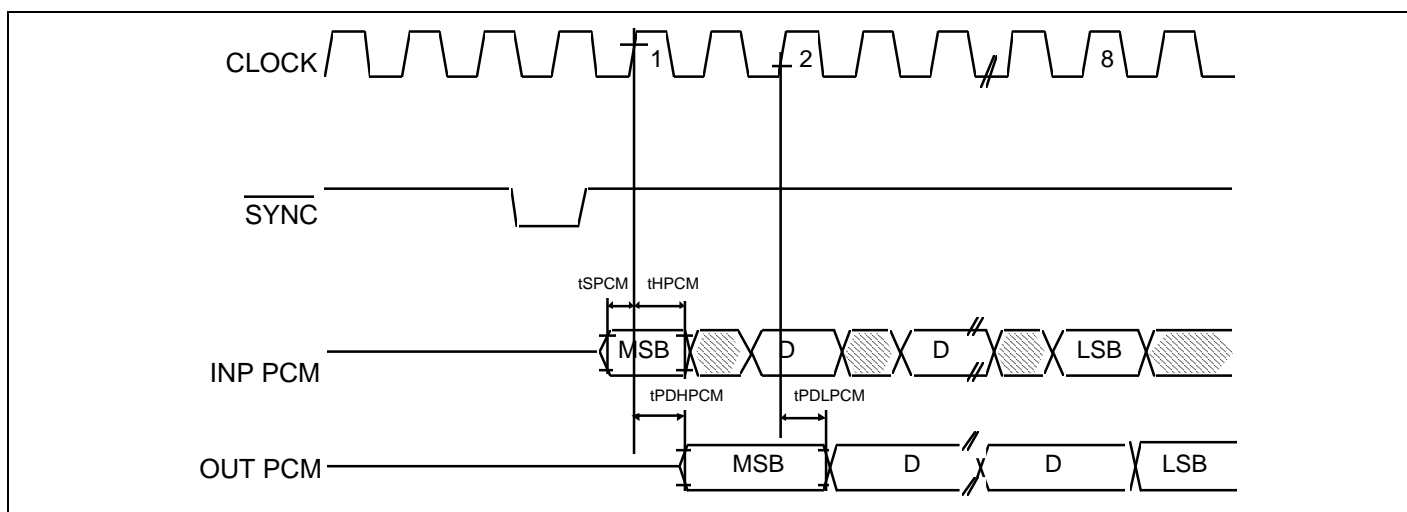
Figure 4. PCM Timing
