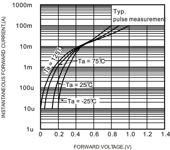
FIG.1-TYPICAL FORWARD CHARACTERISTICS
