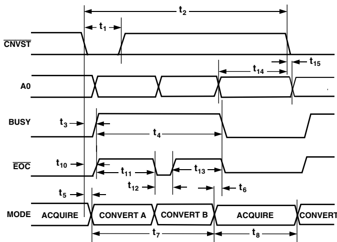
Figure 8. Conversion Control
