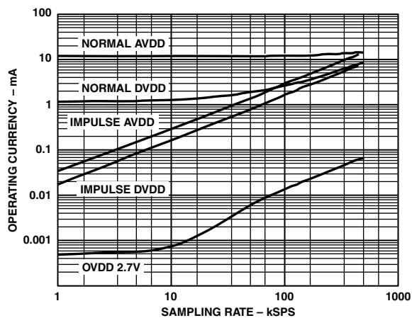
TPC 11. Operating Currents vs. Sample Rate
