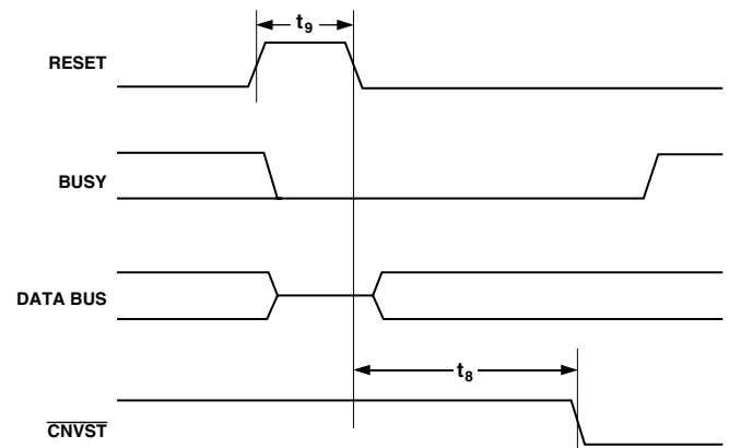
Figure 9. Reset Timing
