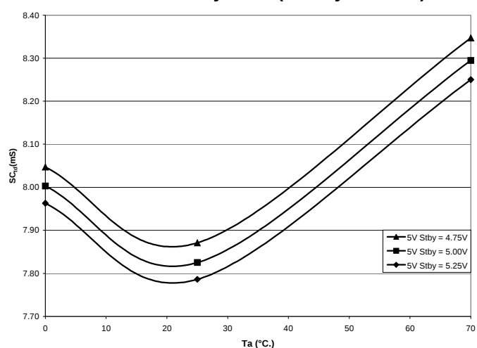
VTT Short circuit Delay Time ( C_{delay} = 0.1\mu F ) vs T_a
