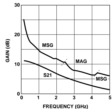
Figure 18. AT-30533 Gains vs. Frequency at V_{CE} = 1\text{ V} , I_C = 1\text{ mA} .
