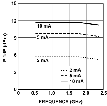
Figure 8. AT-31011 and AT-31033 Power at 1 dB Gain Compression vs. Frequency and Current at V_{CE} = 5\text{ V} .
