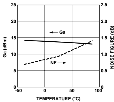
Figure 14. AT-31011 Noise Figure and Associated Gain at V_{CE} = 2.7\text{ V} , I_C = 1\text{ mA} vs. Temperature in Test Circuit, Figure 1. (Circuit Losses De-embedded)
