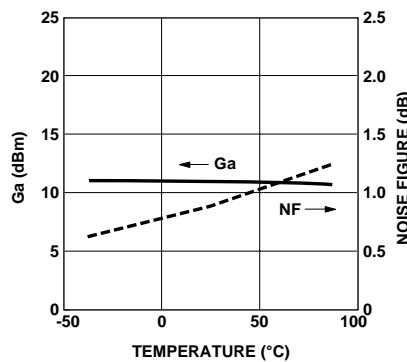
Figure 15. AT-31033 Noise Figure and Associated Gain at V_{CE} = 2.7\text{ V} , I_C = 1\text{ mA} vs. Temperature in Test Circuit, Figure 1. (Circuit Losses De-embedded)
