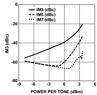
Figure 16. AT-31011 and AT-31033 Intermodulation Products vs. Output Power at V_{CE} = 2.7\text{ V} , I_C = 10\text{ mA} , 900 MHz with Optimal Tuning.
