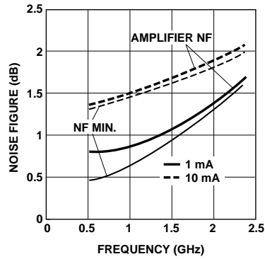
Figure 2. AT-31011 and AT-31033 Minimum Noise Figure and Amplifier NF [1] vs. Frequency and Current at V_{\text{CE}} = 2.7\text{ V} .
