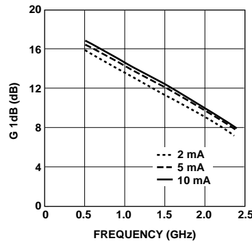
Figure 9. AT-31011 1 dB Compressed Gain vs. Frequency and Current at V_{CE} = 5\text{ V} .
