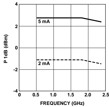
Figure 11. AT-31011 and AT-31033 Power at 1 dB Gain Compression vs. Frequency and Current at V_{CE} = 1\text{ V} .
