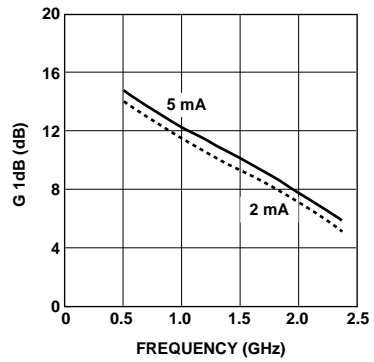
Figure 13. AT-31033 1 dB Compressed Gain vs. Frequency and Current at V_{CE} = 1\text{ V} .
