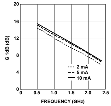
Figure 10. AT-31033 1 dB Compressed Gain vs. Frequency and Current at V_{CE} = 5\text{ V} .
