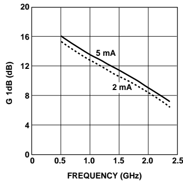
Figure 12. AT-31011 1 dB Compressed Gain vs. Frequency and Current at V_{CE} = 1\text{ V} .
