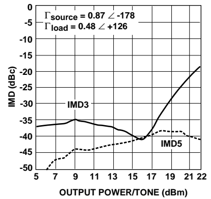
Figure 12. IMD3, IMD5 vs. Output Power Per Tone.
