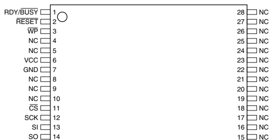
CASON – Top View through Package
