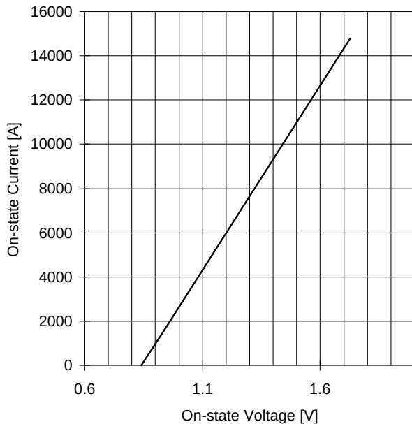
ON-STATE CHARACTERISTIC T_J = 140\text{ }^{\circ}\text{C}
