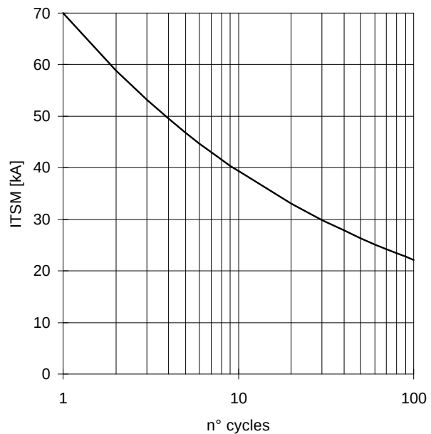
SURGE CHARACTERISTIC T_J = 140\text{ }^{\circ}\text{C}
