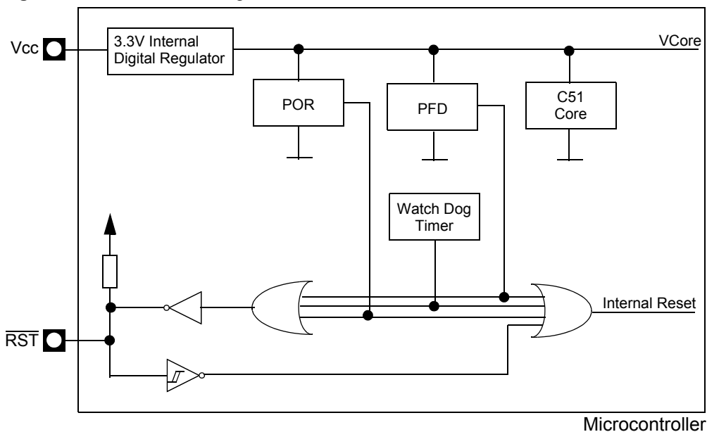
Figure 101. Reset block diagram
