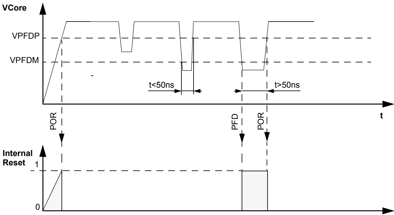
Figure 103. Dynamic behaviour of POR and PFD
