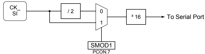
Figure 82. Baud Rate Formula (Mode 2)
