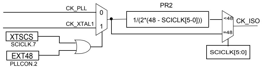
Figure 42. Prescaler 2 Description
