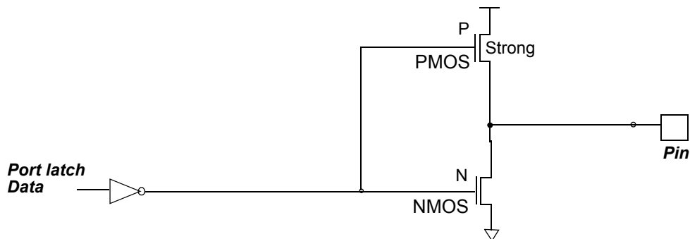
Figure 25. Push-pull Output
