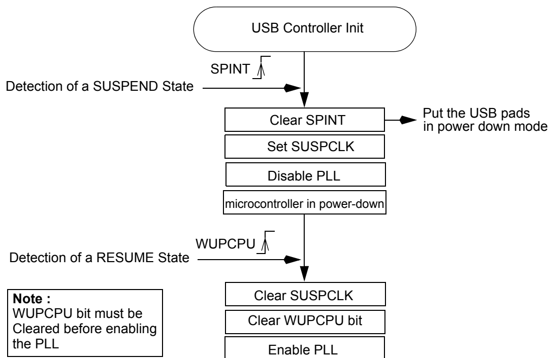
Figure 59. Example of a Suspend/Resume Management
