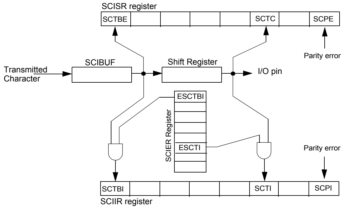
Figure 43. CharacterTransmission Diagram
