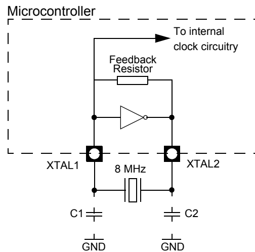
Figure 16. Oscillator Schematic
