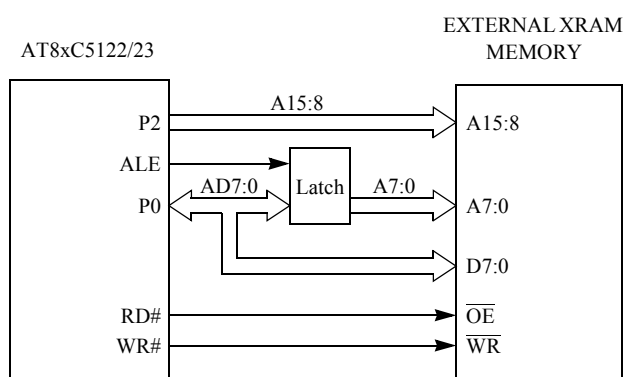
Figure 10. Accessing to External XRAM Memory
