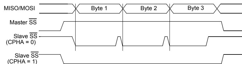
Figure 88. CPHA/SS Timing
