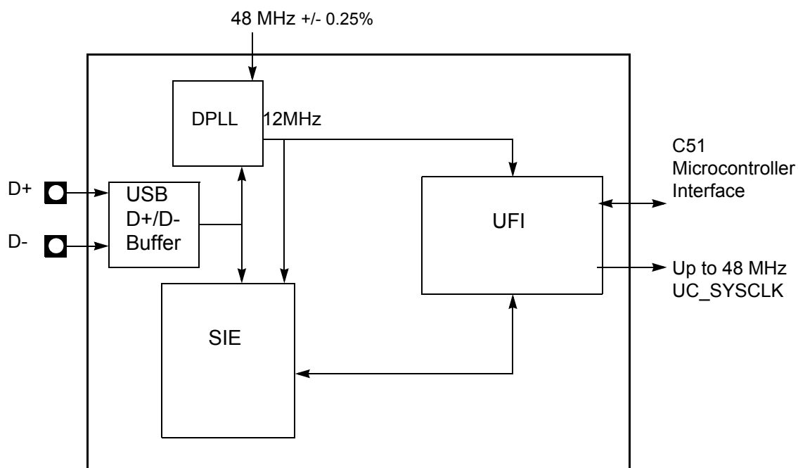
Figure 49. USB Device Controller Block Diagram
