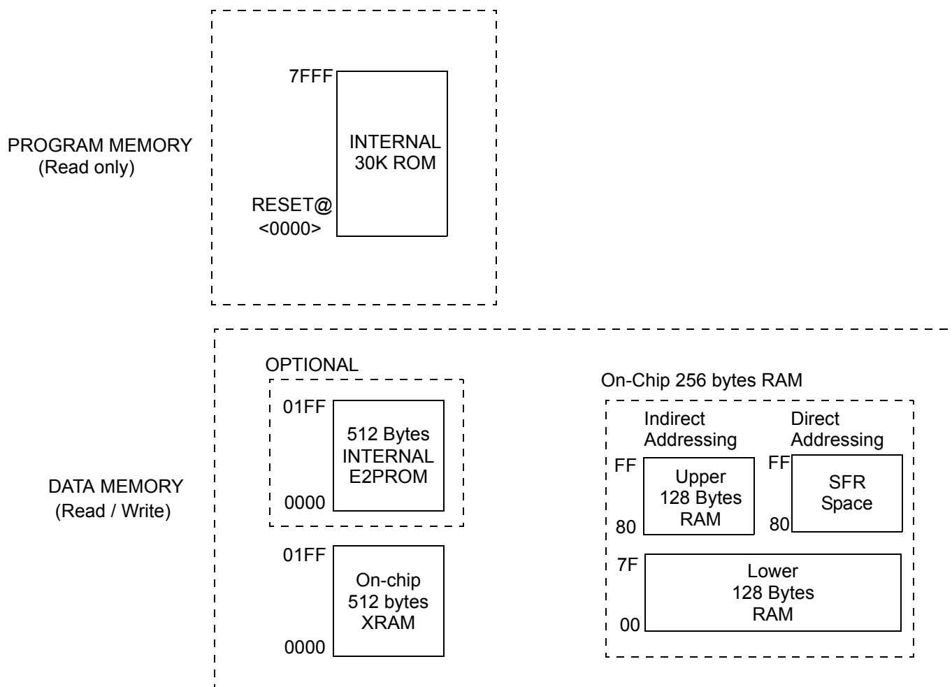
Figure 15. AT83C5123's Device
