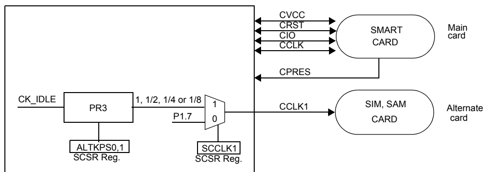
Figure 45. Alternate Card
