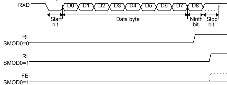
Figure 67. UART Timings in Modes 2 and 3
