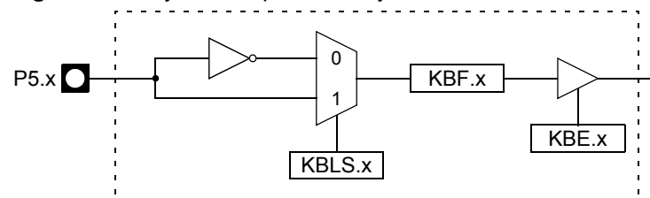
Figure 99. Keyboard Input Circuitry
