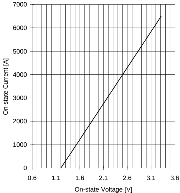
ON-STATE CHARACTERISTIC T_j = 125\text{ }^{\circ}\text{C}
