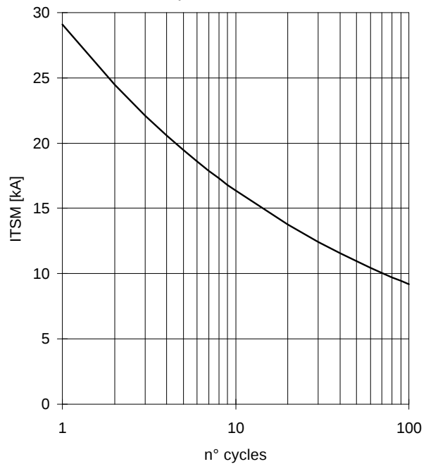
SURGE CHARACTERISTIC T_j = 125\text{ }^{\circ}\text{C}
