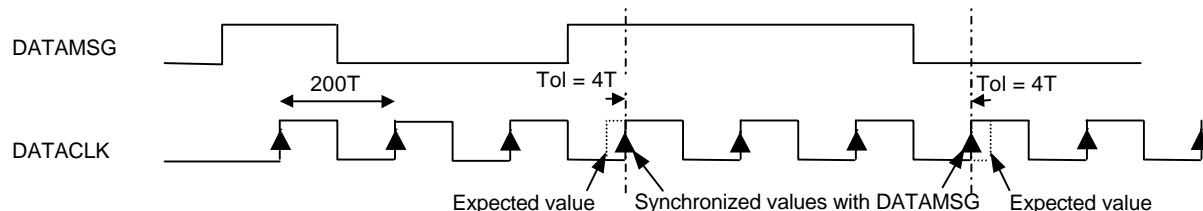
Figure 34. Clock Recovery
