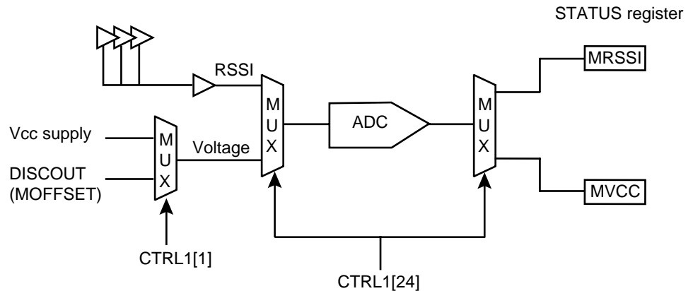
Figure 19. ADC Converter Input Selection
