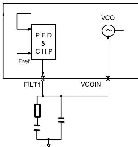
Figure 7. Synthesizer Loop Filter Schematic
