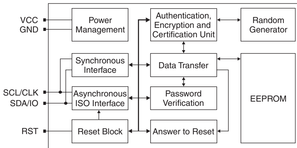
Figure 1. Block Diagram
