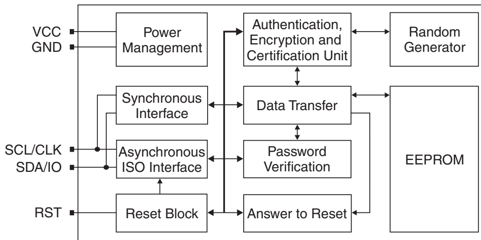
Figure 1. Block Diagram
