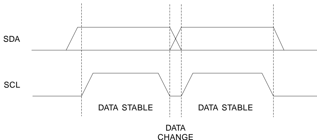
Figure 13. Data Validity
