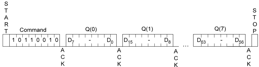
Figure 10. Initiatize Authentication
