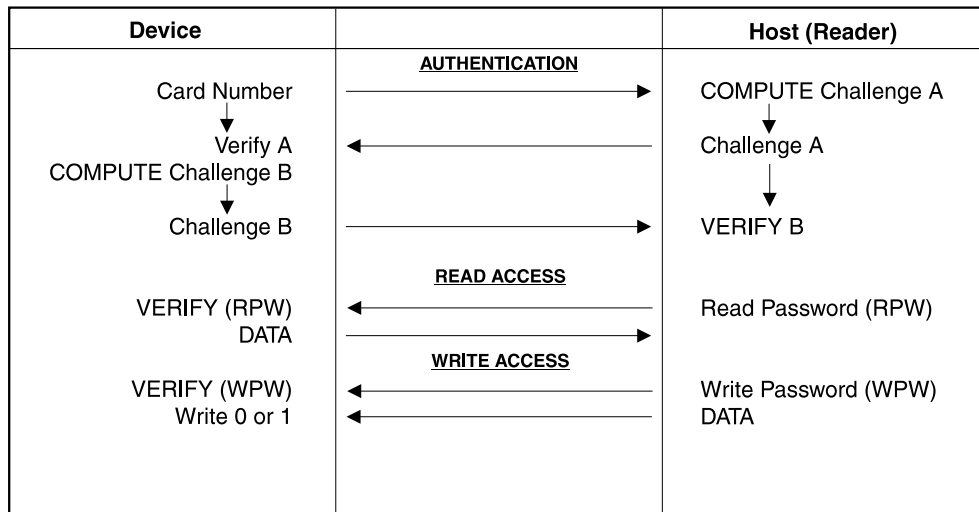
Figure 2. Security Methodology
