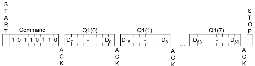
Figure 11. Verify Authentication
