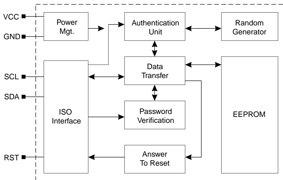
Figure 3. Block Diagram
