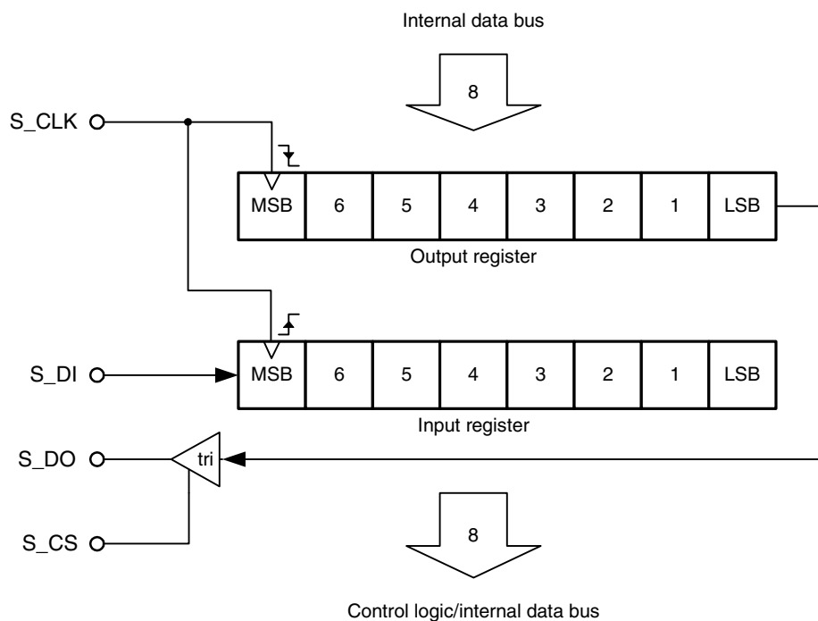
Figure 8. SPI Structure
