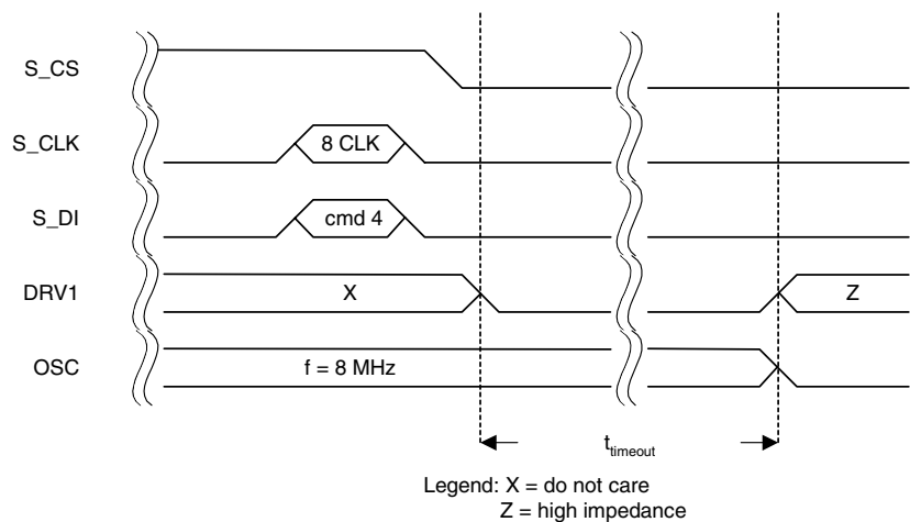
Figure 4. Power-down Timing
