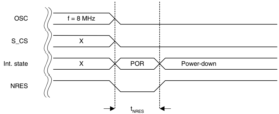
Figure 5. External Reset
