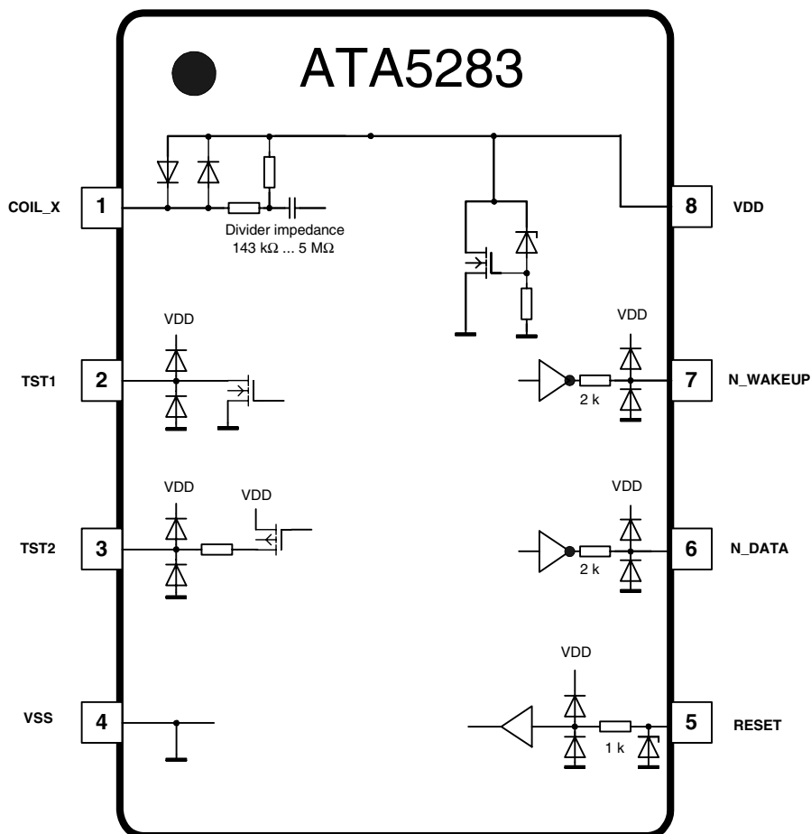
Figure 9. Pin Connection and Pin Protection
