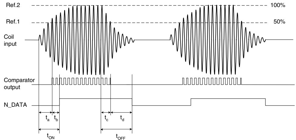
Figure 5. Output Timing
