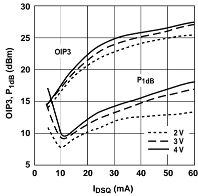
Figure 7. OIP3 and P 1dB vs. Bias at 900MHz. [1,2]
