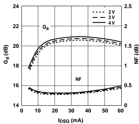
Figure 9. NF and G a vs. Bias at 900MHz. [1]
