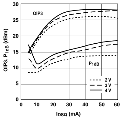
Figure 6. OIP3 and P 1dB vs. Bias at 2GHz. [1,2]
