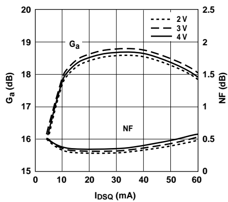
Figure 8. NF and G a vs. Bias at 2GHz. [1]
