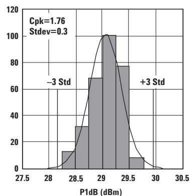
Figure 2. P1dB.
