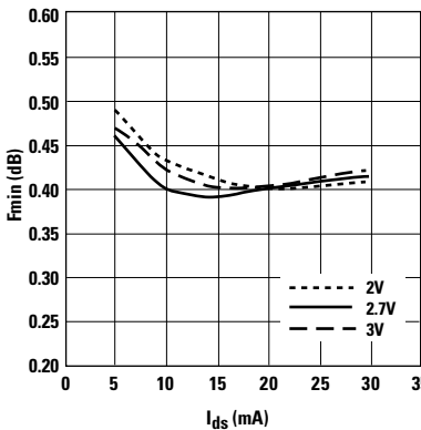
Figure 12. Fmin vs. I_{ds} and V_{ds} at 2 GHz.
