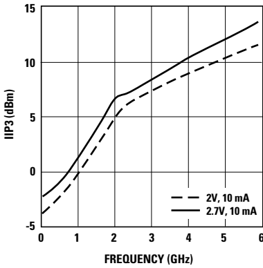
Figure 9. IIP3 vs. Bias over Frequency. [1]
