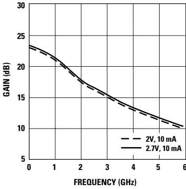
Figure 6. Gain vs. Bias over Frequency. [1]
