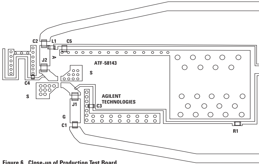
Figure 6. Close-up of Production Test Board.
