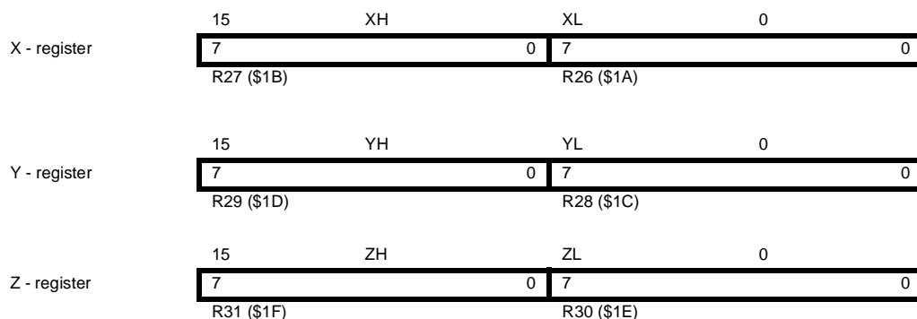
Figure 8. The X-, Y-, and Z-registers
