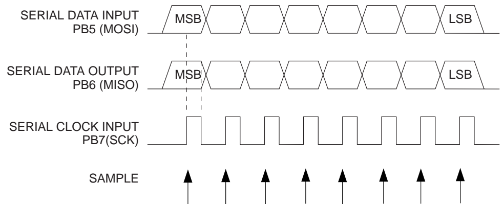
Figure 87. Serial Programming Waveforms
