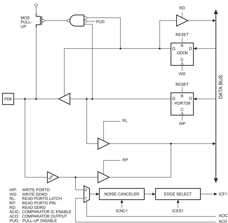
Figure 78. PORTD Schematic Diagram (Pin PD6)
