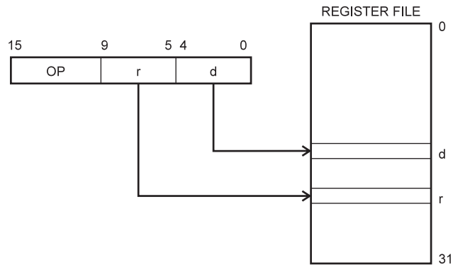
Register Direct, Two Registers Rd And Rr Figure 11. Direct Register Addressing, Two Registers
