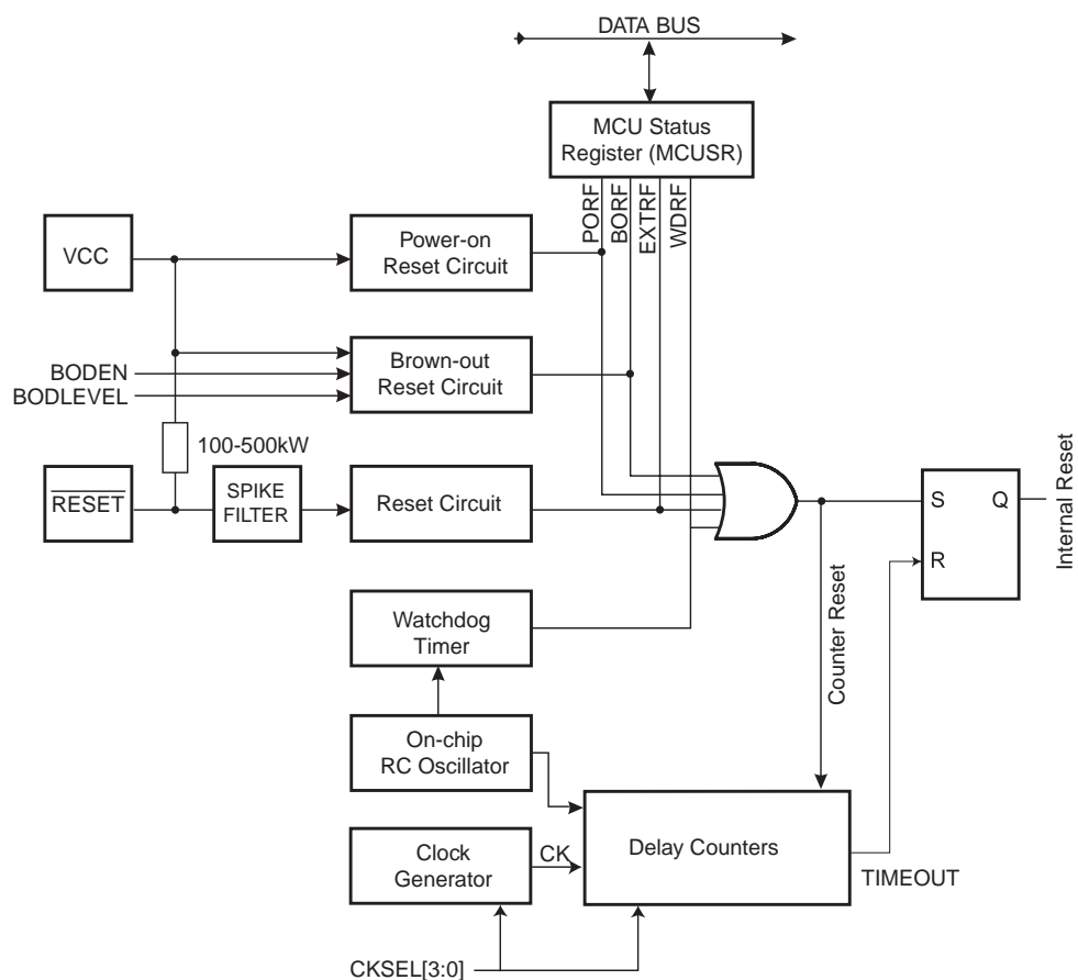
Figure 24. Reset Logic
