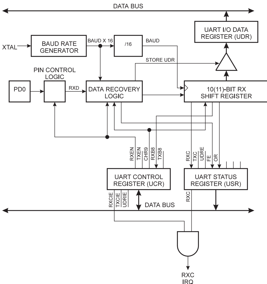
Figure 46. UART Receiver
