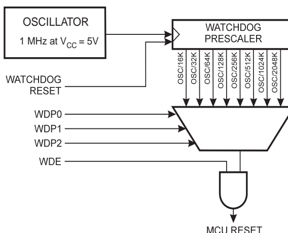
Figure 40. Watchdog Timer
