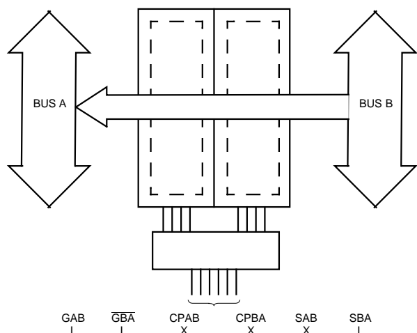
Real-Time Transfer Bus B to Bus A
