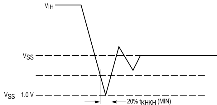
Figure 1. Undershoot Voltage
