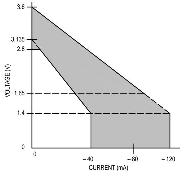
(b) Pull-Up: V_{DDQ} = 3.3 V
