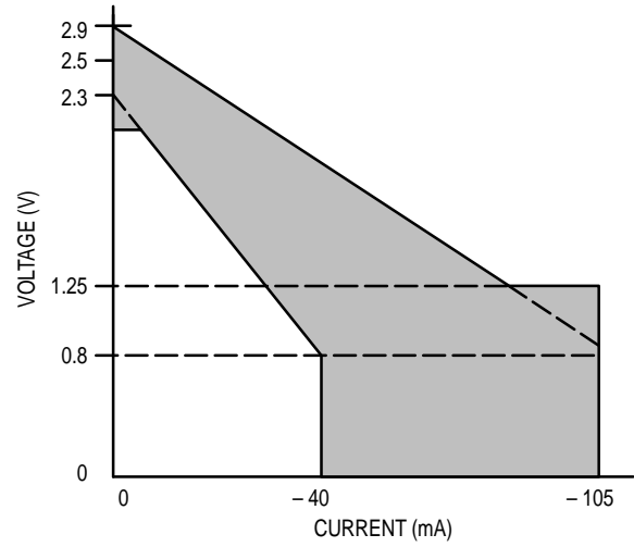
(a) Pull-Up for V_{DDQ} = 2.5 V
