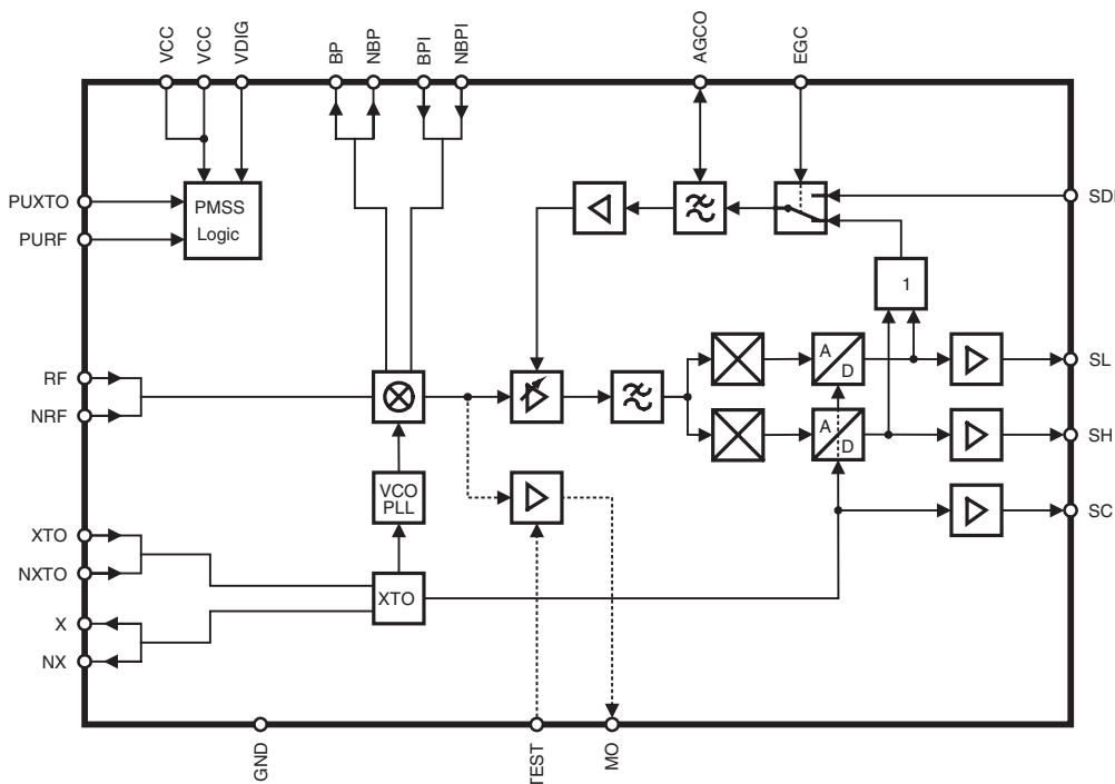
Figure 1-1. Block Diagram
