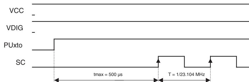
Figure 8-4. Sample Clock Start-up Delay
