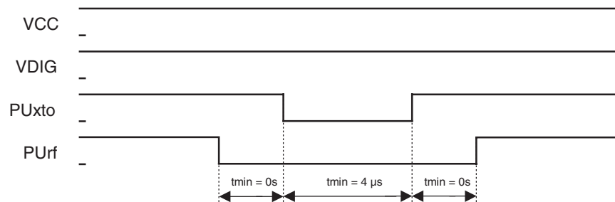
Figure 8-2. Recommended Sleep-mode Sequence
