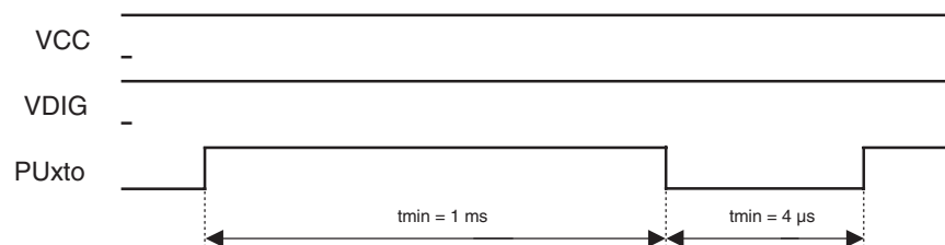
Figure 8-3. Recommended XTO Start-up/Shut-down Sequence
