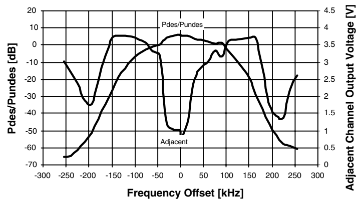
Figure 18. Selectivity
