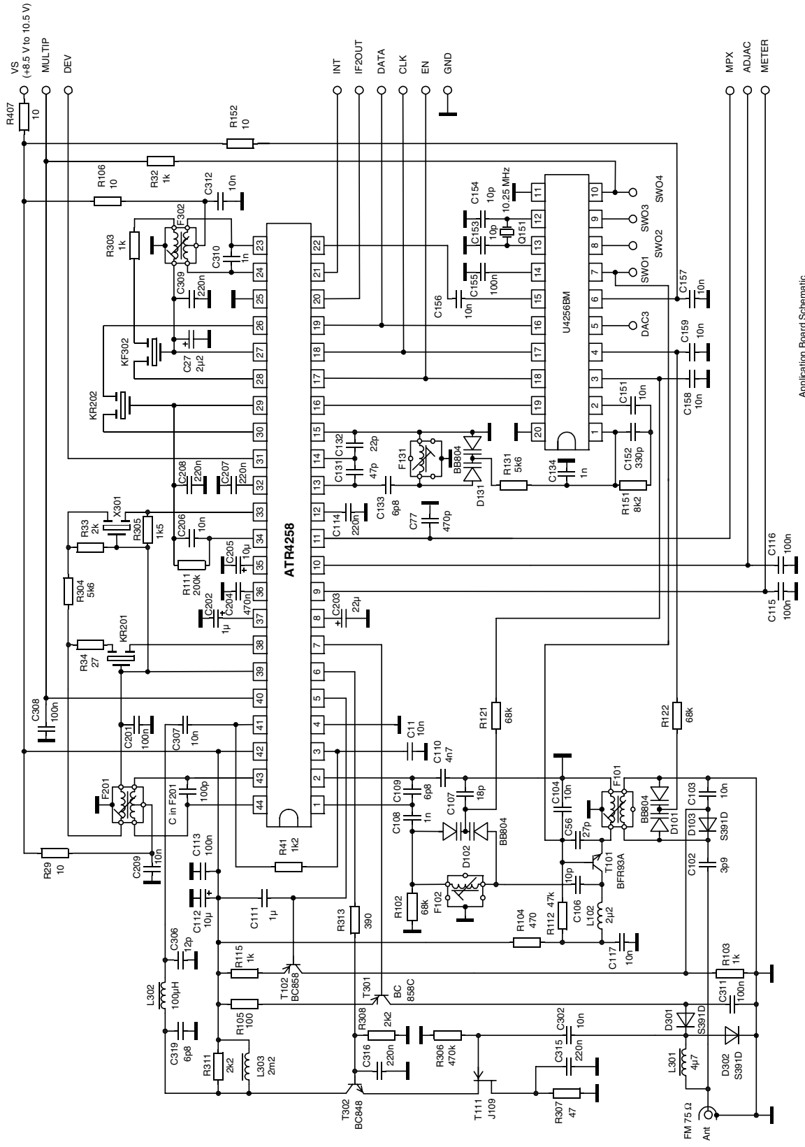
Figure 20. Application Circuit
