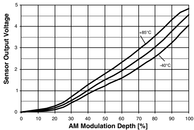
Figure 13. Multipath Sensor
