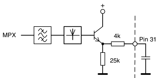
Figure 7. Deviation Sensor
