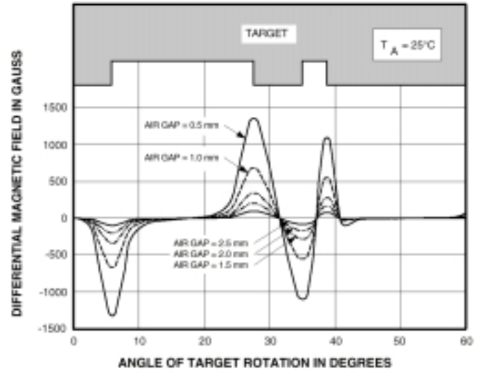
Differential flux maps vs. air gaps
