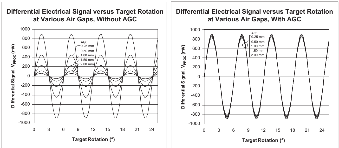
Figure 7. Effect of AGC. The left panel shows the process signal, V_{PROC} , without AGC. The right panel shows the effect with AGC. The result is a normalized V_{PROC} , which allows optimal performance by the rest of the circuits that reference this signal.
