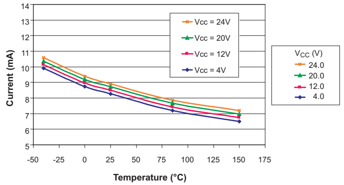
I CC(OFF) Versus T A
