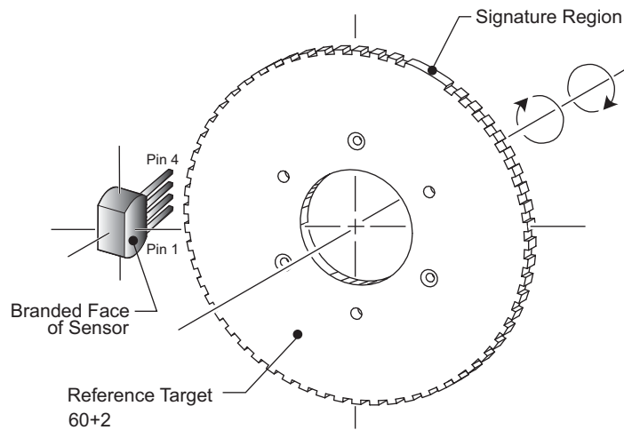
Figure 1. Configuration with Spur Gear Reference Target
