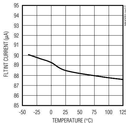
FLTINT CURRENT vs. TEMPERATURE
