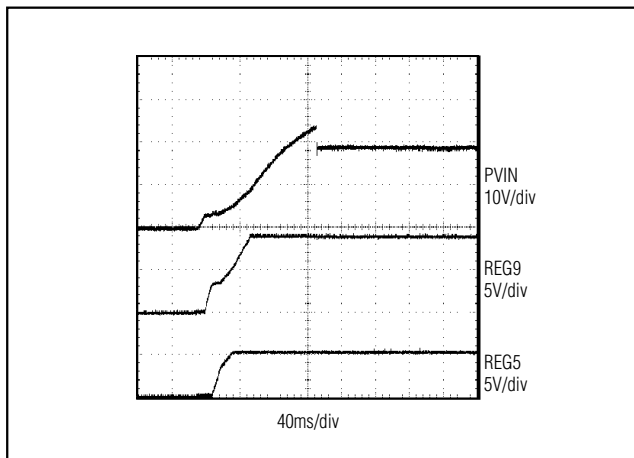
Figure 6. PVIN, REG5, and REG9 During Startup in Bootstrapped Mode
