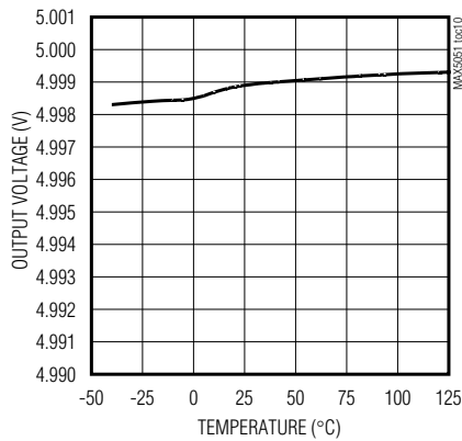
REG5 OUTPUT VOLTAGE vs. TEMPERATURE
