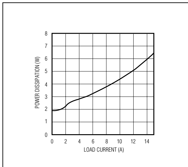
Figure 10. Power Dissipation at Nominal Output Voltage vs. Load Current for 48V Input Voltage.
