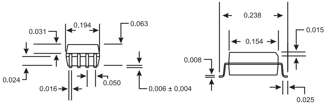
8-Pin Plastic SOIC Package
