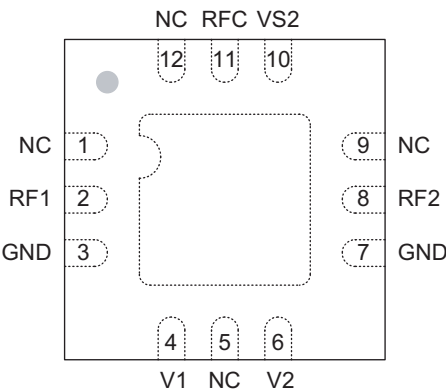
Figure 3: Packaged Device Pinout (X-ray Top View)
