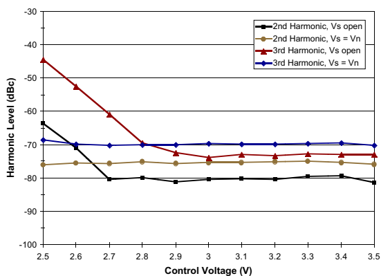
Figure 13: Harmonics of 2 GHz vs. Control Voltage Packaged Device (ON path, V_x = 0 V, f = 2 GHz, P_{IN} = +32 dBm)
