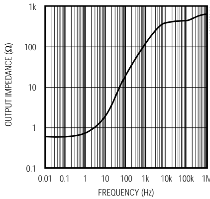
MAX6005 OUTPUT IMPEDANCE vs. FREQUENCY
