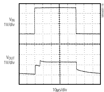
MAX6001 TURN-ON TRANSIENT
