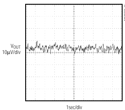
MAX6001 0.1Hz TO 10Hz OUTPUT NOISE
