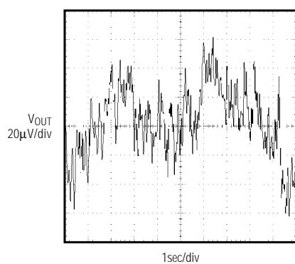
MAX6005 0.1Hz TO 10Hz OUTPUT NOISE
