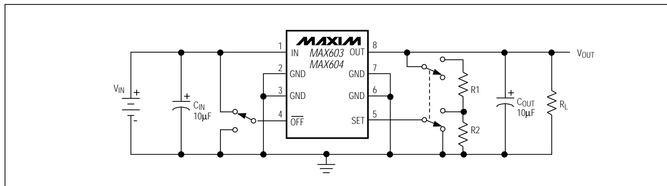
Figure 1. Test Circuit
