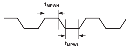
Figure 3. MCLK_I Timing
