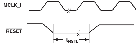
Figure 2. \overline{RESET} Timing
