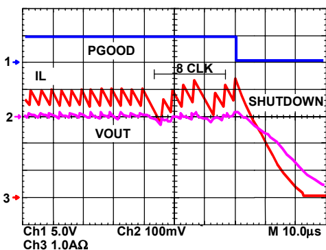
FIGURE 8. OVERCURRENT PROTECTION
