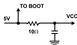
FIGURE 9. INPUT FILTERING FOR THE CHIP
