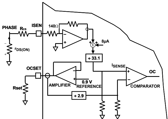
FIGURE 10. EQUIVALENT CIRCUIT FOR OC SIGNAL GENERATOR
