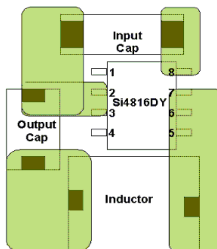
FIGURE 11. A GOOD EXAMPLE POWER COMPONENT REPLACEMENT. IT SHOWS THE NEGATIVE OF INPUT AND OUTPUT CAP AND THE SOURCE OF THE MOSFET ARE TIED AT ONE POINT.
