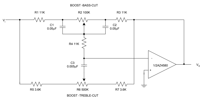
Figure12. Tone Control
