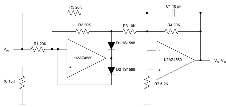
Figure 10. AC/DC Converter
