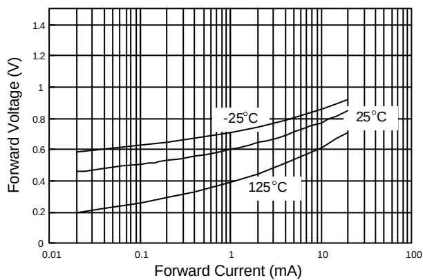
Fig. 3 Forward Characteristics
