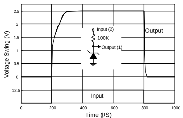
Fig. 4 Response Time
