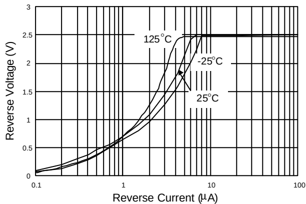
Fig. 1 Reverse Characteristics
