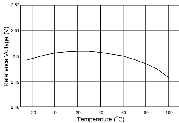
Fig. 5 Temperature Drift
