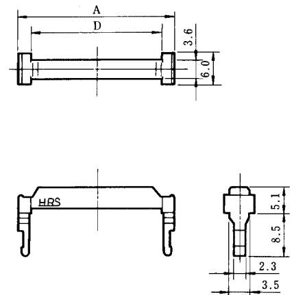
Clamp
