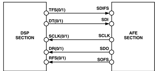
Figure 8. Indirectly Coupled or Nonframe Sync Loop-Back Configuration
